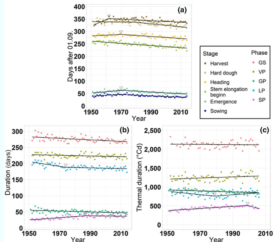
FIGURE 5 Estimated phenology trends of winter wheat across the study sites between 1951 and 2015. (a) Average days of sowing, harvest and the actual crop phenological stages (emergence, begin of stem elongation, heading and hard dough) after 1 September. Average duration (b) and thermal duration (c) of the entire growing season (GS) divided into the generative phase (GP) and vegetative phase (VP). The latter comprises the leaf development phase (LP) and the stem elongation phase (SP). Inverse triangles indicate trend changes
