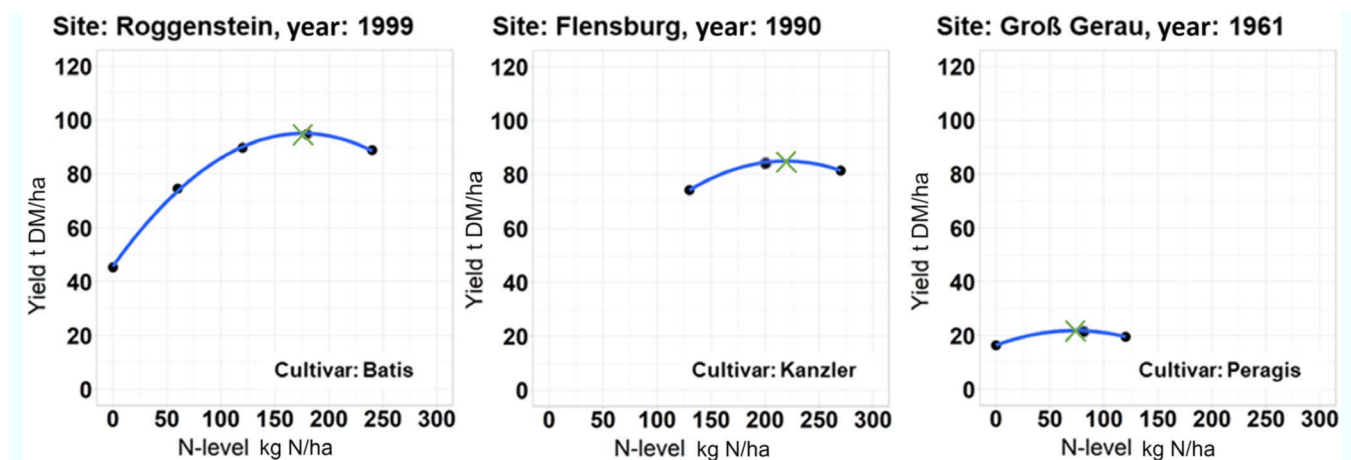
FIGURE 2 Examples for the yield response curves to nitrogen fertilizer level and derived maximum yields and corresponding nitrogen values of three fertilization experiments. The green crosses mark the maximum achievable winter wheat yields as derived from a quadratic linear function and its corresponding nitrogen level
